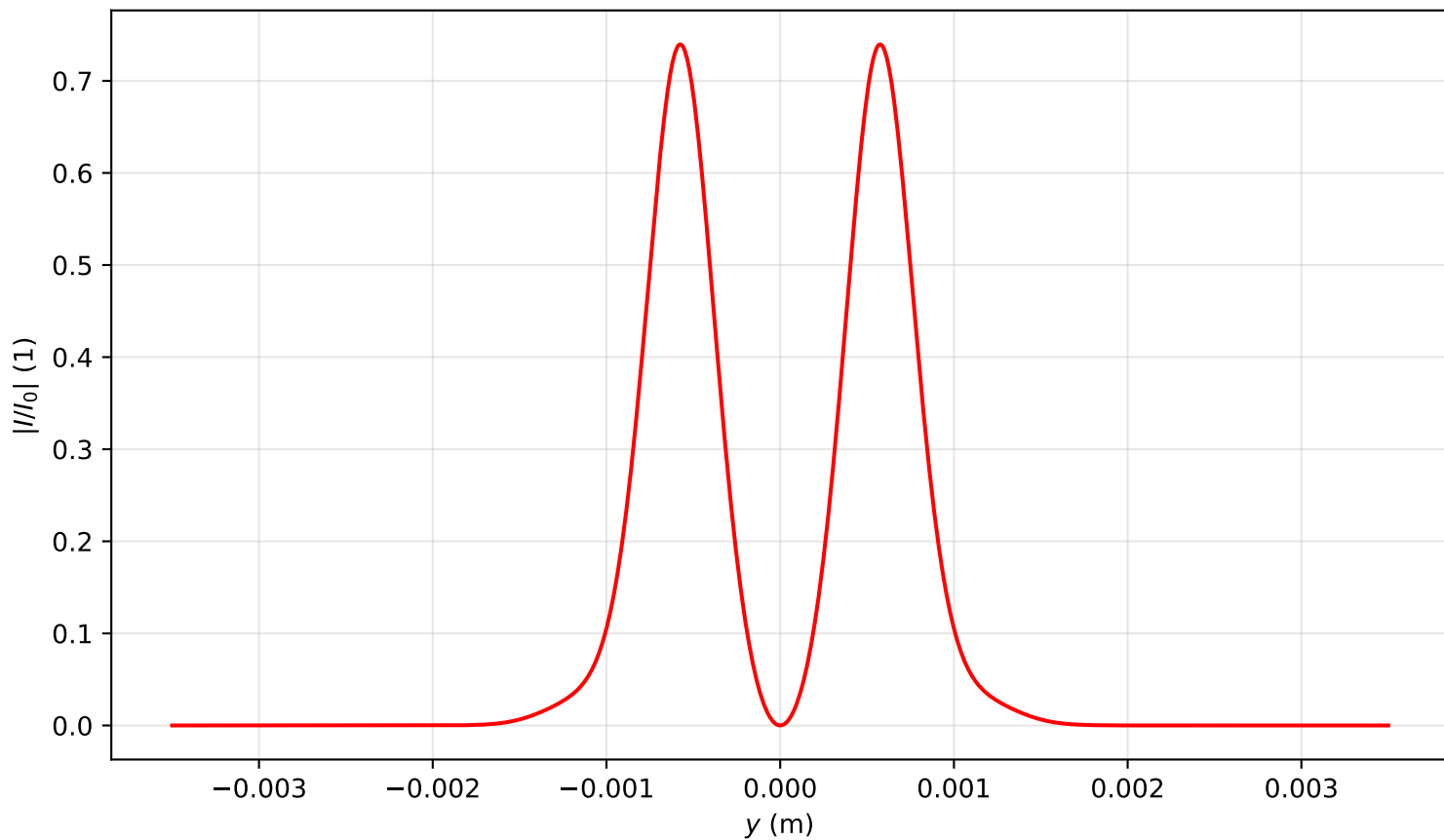
Intensity profile I(x=0, y, z=0.876)/I_0 , P_{in}=3.0P_{cr} , artificial time
